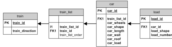
Fig. 3. East-West-Challenge as a relational database.
